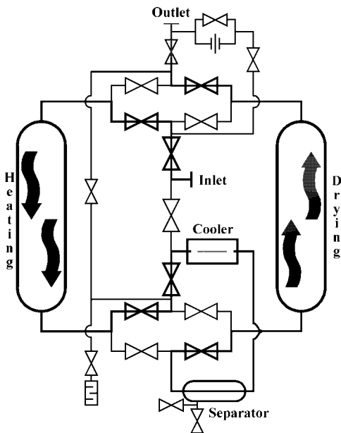
Illustration 9: Heat-of-Compression Heating Cycle
