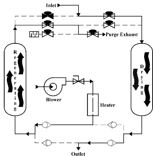
Illustration 6: Blower Purge Flow Schematic
