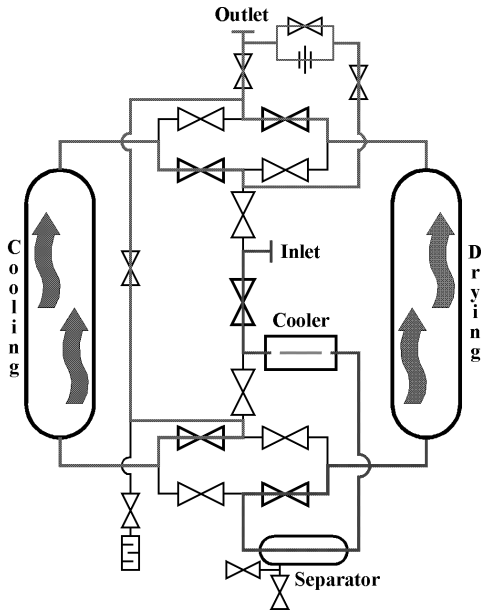
Illustration 11: Heat-of-Compression Cooling Cycle
